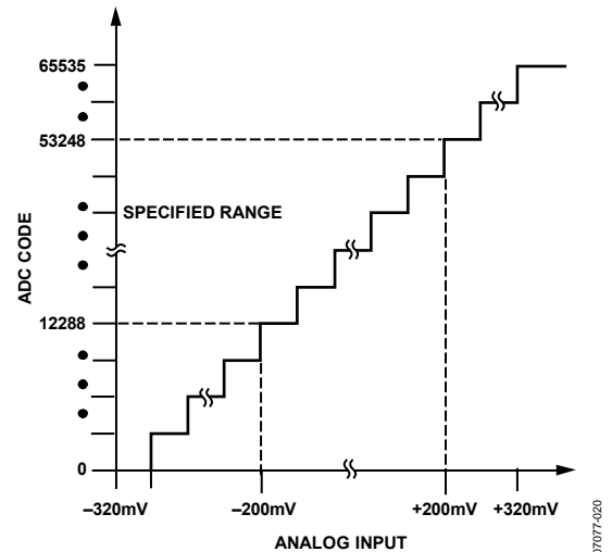
Figure 20. Filtered and Decimated 16-Bit Transfer Characteristic
