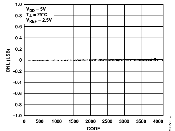
Figure 14. AD5691R DNL
