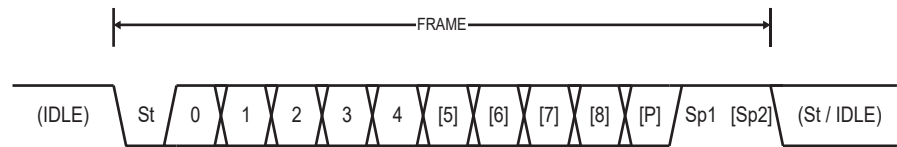
Figure 22-4. Frame Formats
