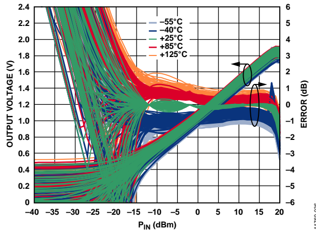
Figure 31. Distribution of Log Conformance Error with Respect to Calibration at 25°C vs. Input Level and Temperature at 5.8 GHz
