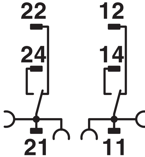
Circuit diagram
