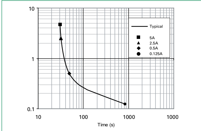
Fig. 1 Typical time to open circuit under UL1449 Abnormal Overvoltage Limited Current Test
