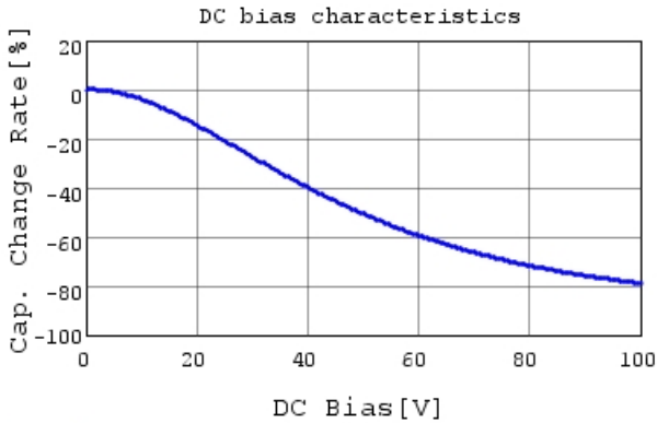
RDER72A105K2P1H03B C-DC bias capchange, 25.0
