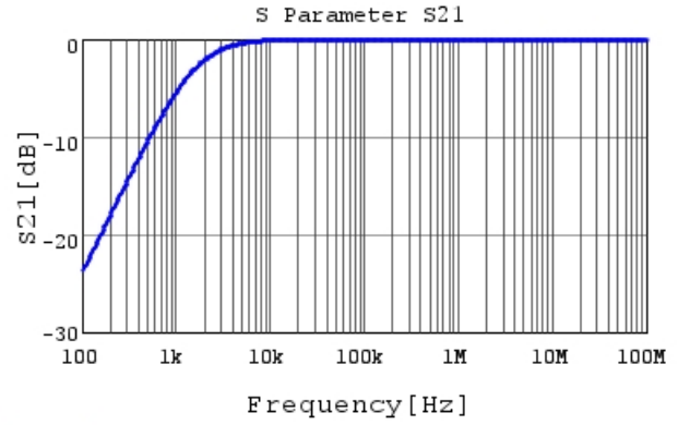
RDER72A105K2P1H03B S21 DC0V, 25degC
