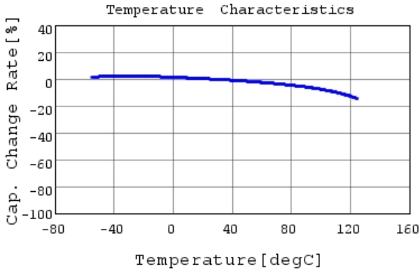
RDER72A105K2P1H03B C-Temp. capchange, DC0.0V
