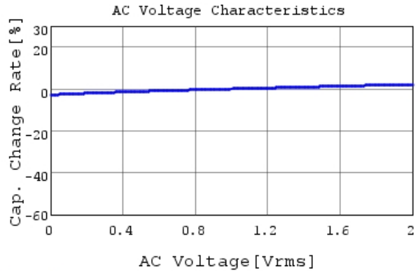
RDER72A105K2P1H03B C-AC Voltage capchange, I
