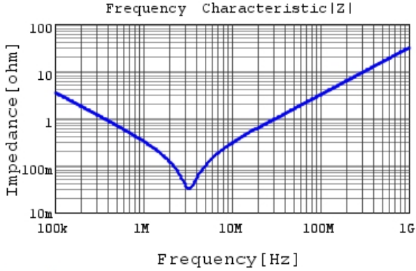
RDER72A474K1M1H03A |Z| DCOV, 25degC
