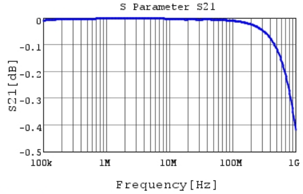
RDER72A474K1M1H03A S21 DC0V, 25degC
