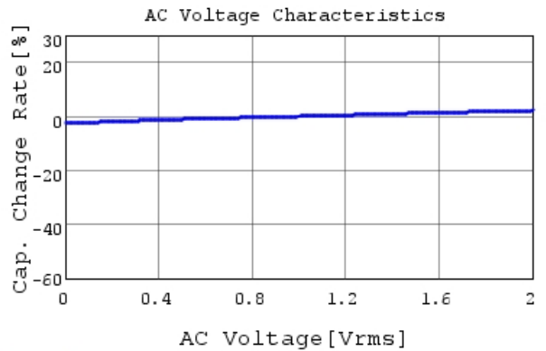
RDER72A474K1M1H03A C-AC Voltage capchange, I
