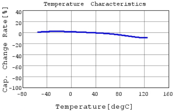
RDER72A474K1M1H03A C-Temp. capchange, DC0.0V
