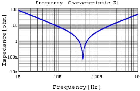
RDE5C1H222J0M1H03A |Z| DCOV, 25degC
