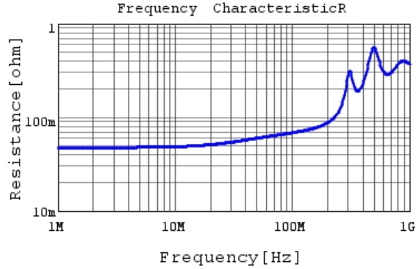
RDE5C1H222J0M1H03A R DCOV, 25degC
