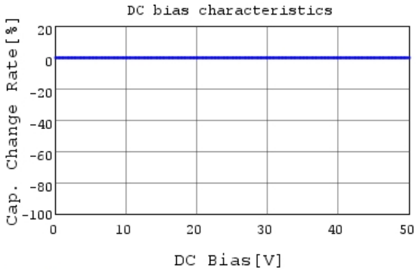
RDE5C1H222J0M1H03A C-DC bias capchange, 25.0
