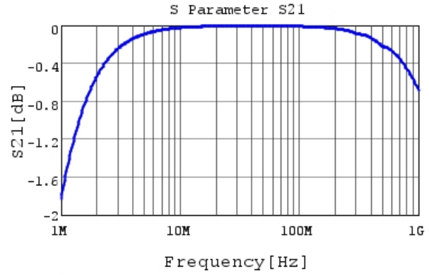
RDE5C1H222J0M1H03A S21 DCOV, 25degC
