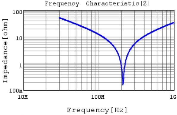
RDE5C1H101J0S1H03A |Z| DC0V, 25degC
