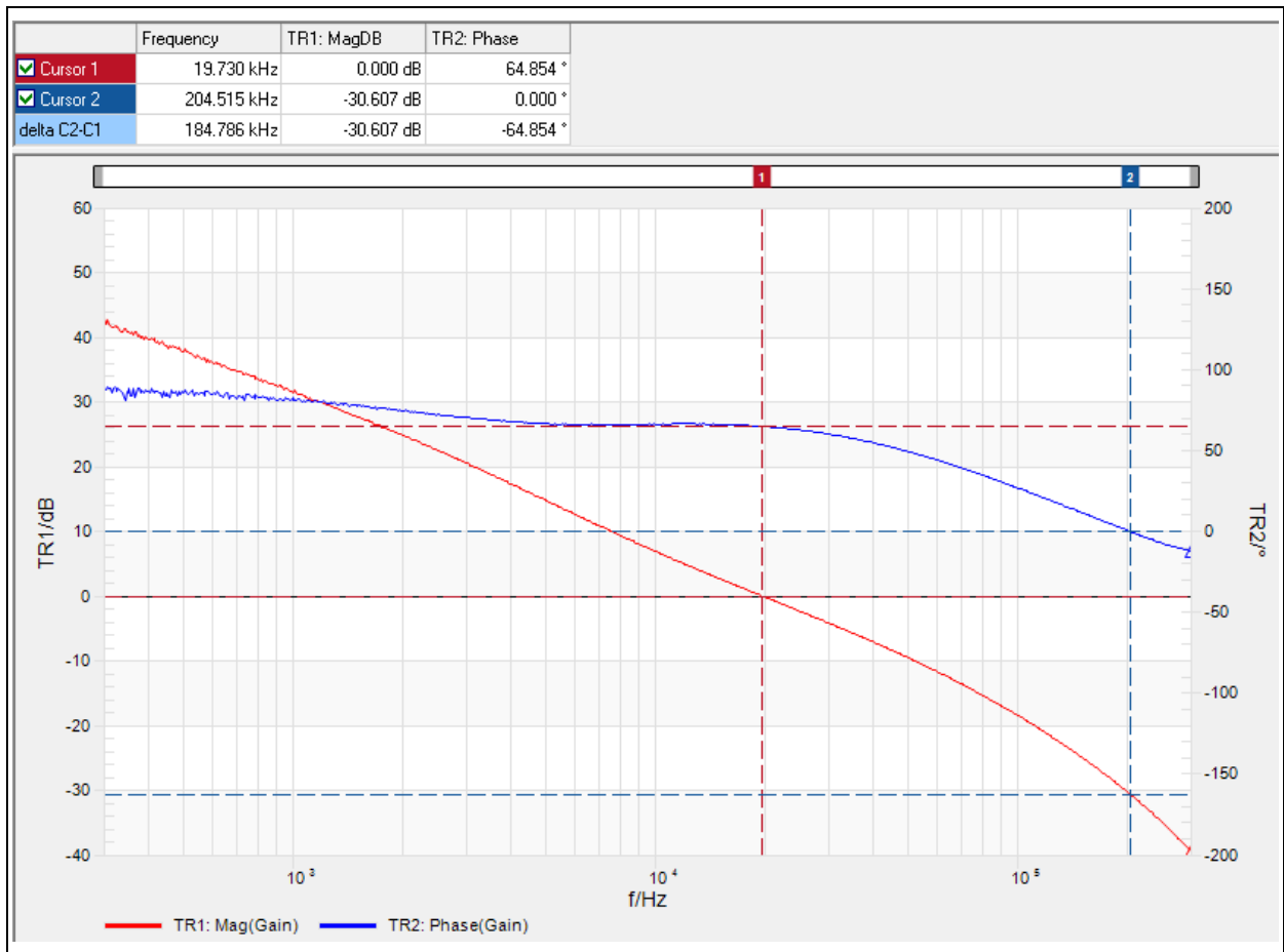
FIGURE 2-40: Voltage Loop Gain Bode Plot, V_{OUT} = 1.8V , f_s = 570\text{ kHz} , L = 1.2\ \mu\text{H} , C_{OUT} = 266\ \mu\text{F} , R_{C1} = 2.55\text{k}\Omega , C_{C1} = 10\text{nF} , C_{C2} = 47\text{pF} (see Section 7.7, Compensation Design ).
