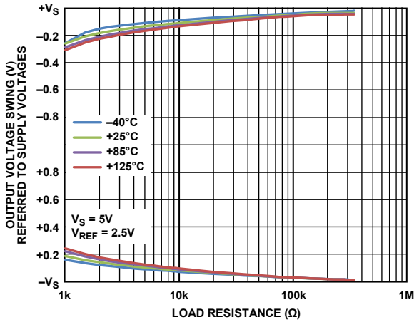
Figure 39. Output Voltage Swing vs. Load Resistance, V_S = 5V
