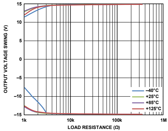
Figure 41. Output Voltage Swing vs. Load Resistance, V_S = \pm 15V
