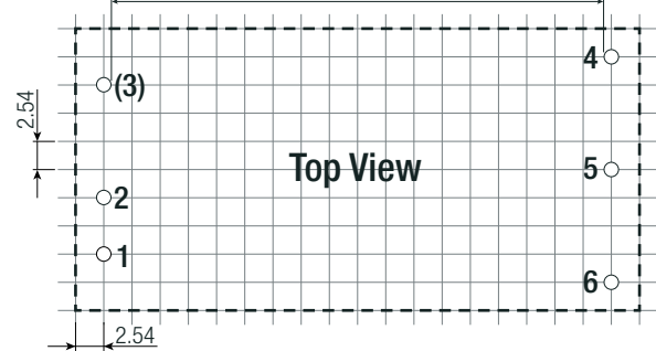
Recommended Footprint Details creepage= 8mm min. *
