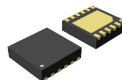
DFN3030-12 3.0 x 3.0 x 0.8 (1) mm (1) maximum dimension
