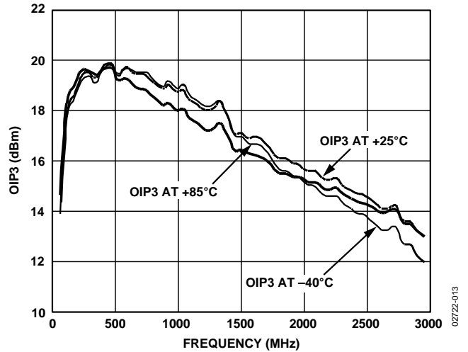
Figure 14. OIP3 vs. Frequency, V S = 3 V, T A = -40°C, +25°C, and +85°C
