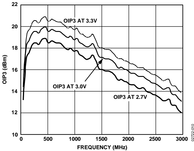
Figure 11. OIP3 vs. Frequency, V S = 2.7 V, 3 V, and 3.3 V, T A = 25°C
