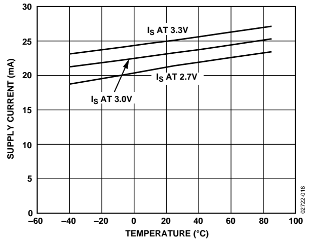
Figure 19. Supply Current vs. Temperature, V_S = 2.7\text{ V}, 3\text{ V}, \text{ and } 3.3\text{ V}
