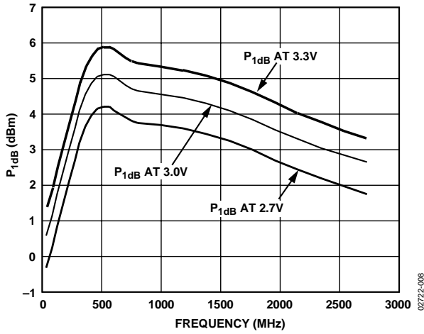
Figure 9. P 1dB vs. Frequency, V S = 2.7 V, 3 V, and 3.3 V, T A = 25°C
