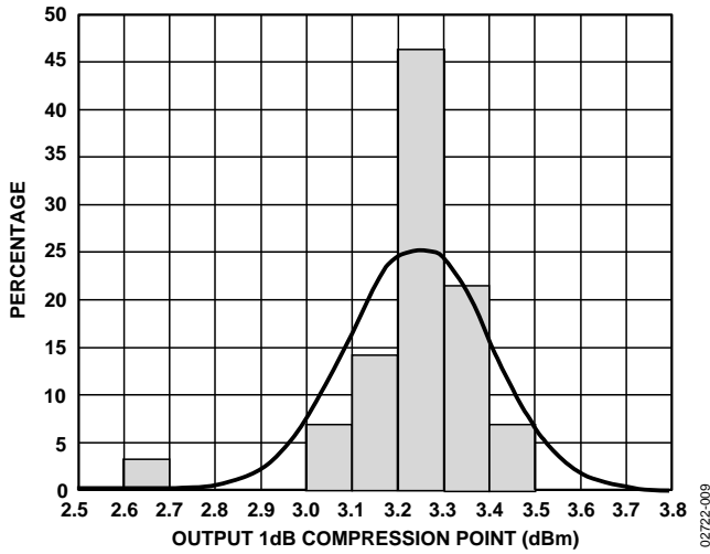
Figure 10. Distribution of P 1dB , V S = 3 V, T A = 25°C, f = 2.2 GHz
