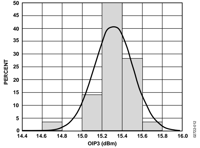
Figure 13. Distribution of OIP3, V S = 3 V, T A = 25°C, f = 2.2 GHz
