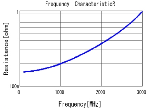
■ GRM31A5C2J220JW01 R DC0V, 25degC
