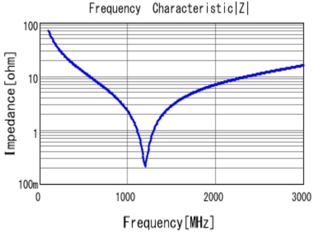
■ GRM31A5C2J220JW01 |Z| DC0V, 25degC
