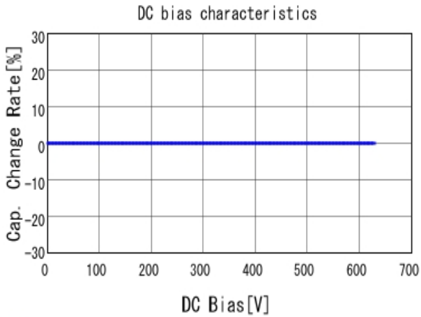
■ GRM31A5C2J220JW01 C-DC bias capchange, 25.0degC, AC1V
