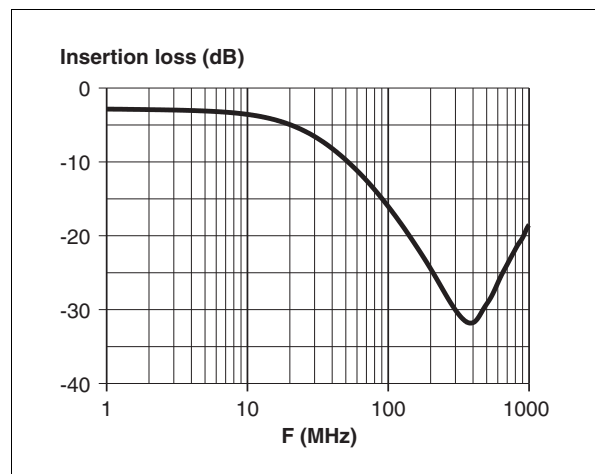
Figure 3: KBMF attenuation curve
