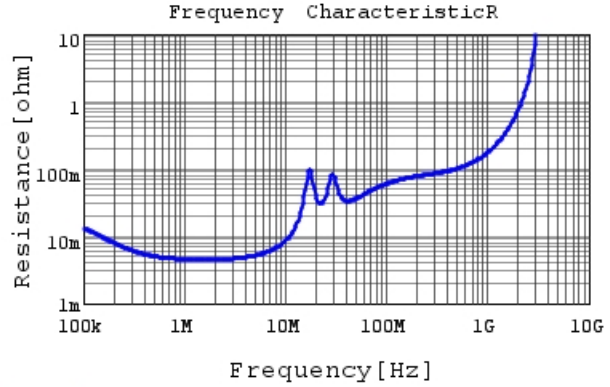
GR355DD72W474KW01 R DCOV, 25degC
