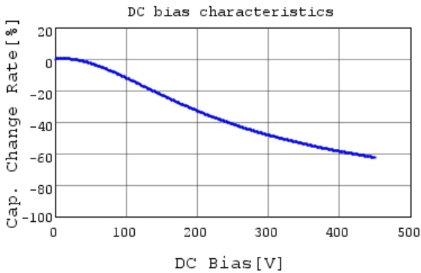
GR355DD72W474KW01 C-DC bias capchange, 25.0c
