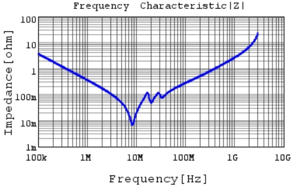
GR355DD72W474KW01 |Z| DCOV, 25degC
