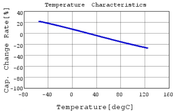
GR355DD72W474KW01 C-Temp. capchange, DCOV, 1
