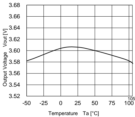
R1180x361x ( V_{IN}=4.6V )
