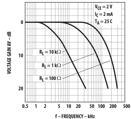
Figure 11: Frequency Response
