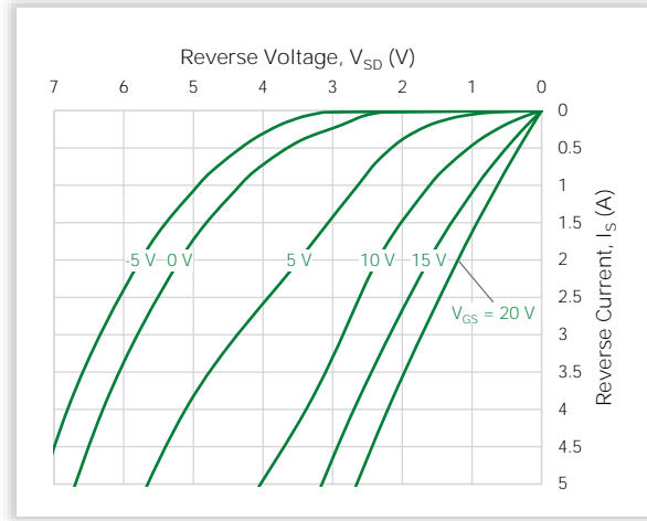
Figure 8. Typical Reverse Conduction Characteristics ( T_J = -55\text{ }^\circ\text{C} )
