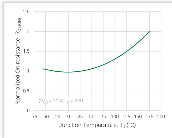
Figure 12. Normalized On-resistance vs. Junction Temperature
