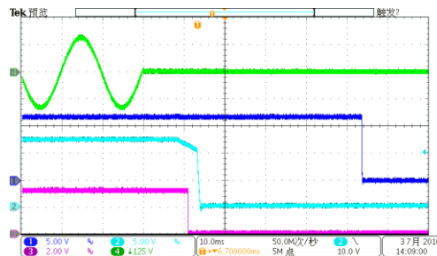
Figure 6. Turn-Off AC Line 230VAC, full load (10ms/div)
