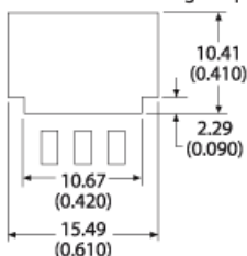
Recommended copper pad size for heat sink and device mounting footprint
