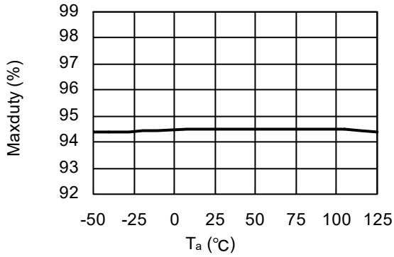
R1245x00xA/R1245x00xB ( V_{IN}=12V )
