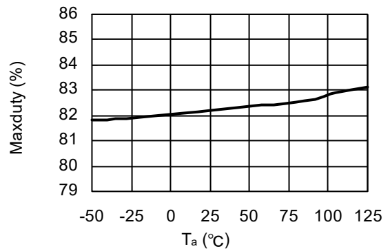
R1245x00xG/R1245x00xH ( V_{IN}=12V )
