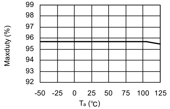
R1245x00xC/R1245x00xD ( V_{IN}=12V )
