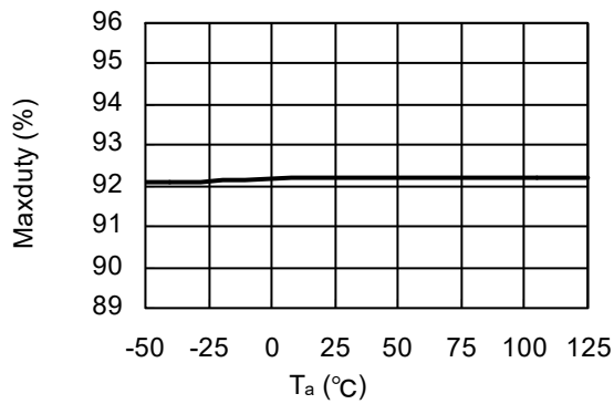
R1245x00xE/R1245x00xF ( V_{IN}=12V )
