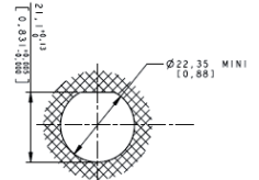
PANEL DRILLING
