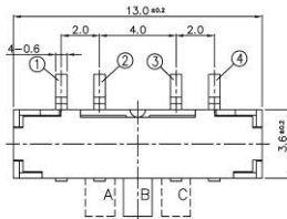
Outline Drawing
