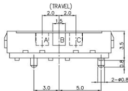
Mounting
