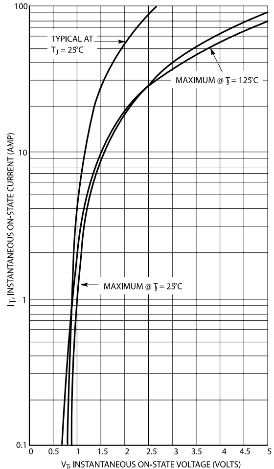
Figure 3. On-State Characteristics
