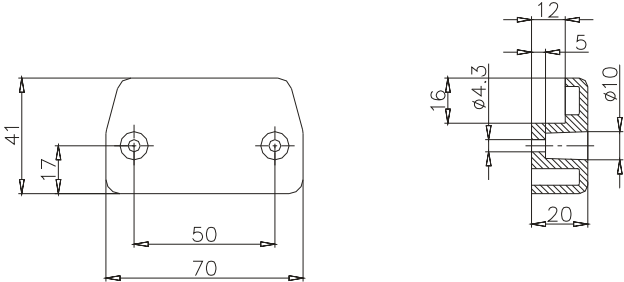
Wall holder Set complete with 2 fittings and screws Order No. 29. 60 01 00
