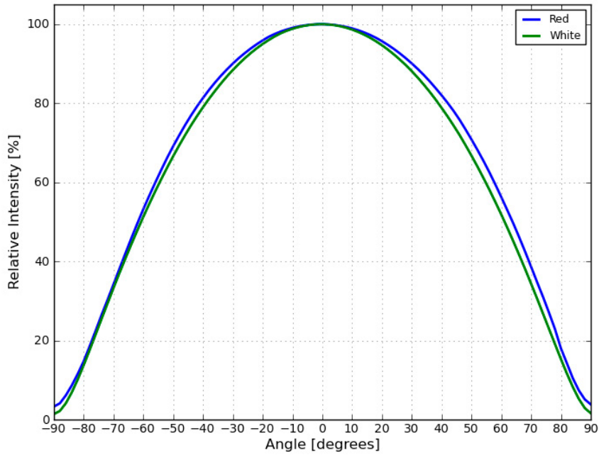
Figure 5a. Typical radiation pattern for LUXEON Rubix Red and White at 1500mA, T_j=85^\circ\text{C} .
