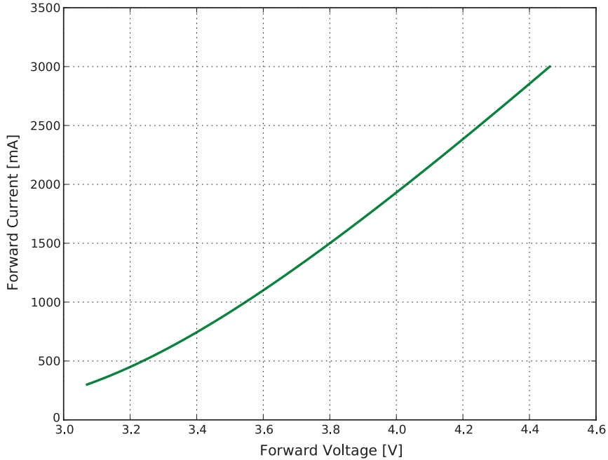
Figure 4b. Typical forward current vs. forward voltage for LUXEON Rubix Green at T_j=85^\circ\text{C} .
