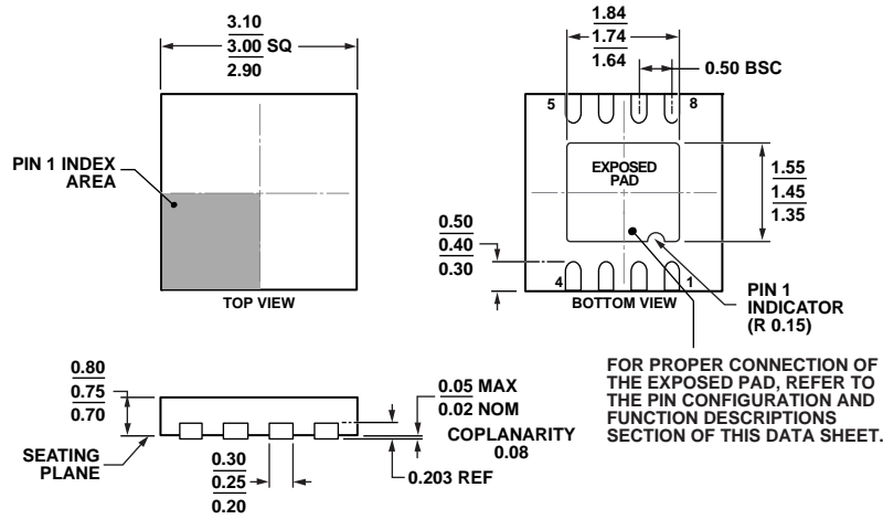
Figure 41. 8-Lead Lead Frame Chip Scale Package [LFCSP] 3 mm x 3 mm Body and 0.75 mm Package Height (CP-8-13) Dimensions shown in millimeters
