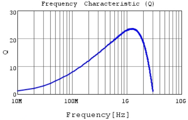
LQP03TN22NJ02 Q
