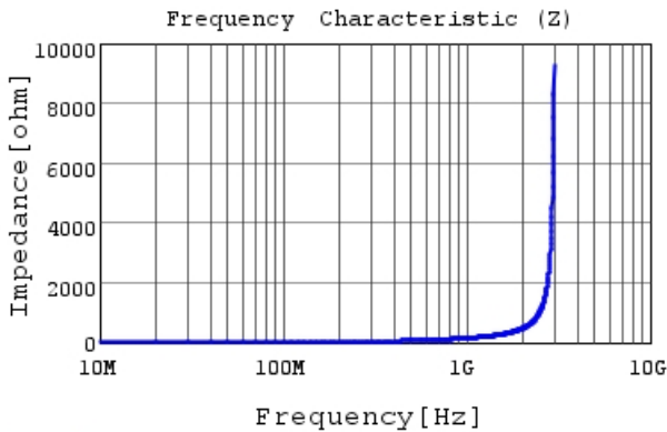
LQP03TN22NJ02 |Z|
