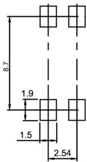
SOP4 (Top View)
