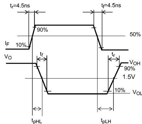
Fig. 12.1.5 Switching Time Test Circuit and Waveform
