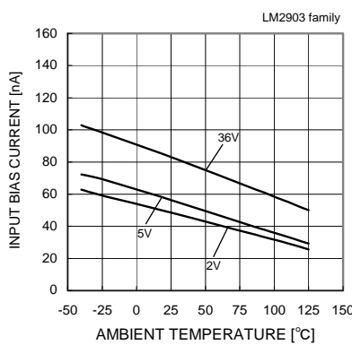
Fig. 51 Input Bias Current - Ambient Temperature
