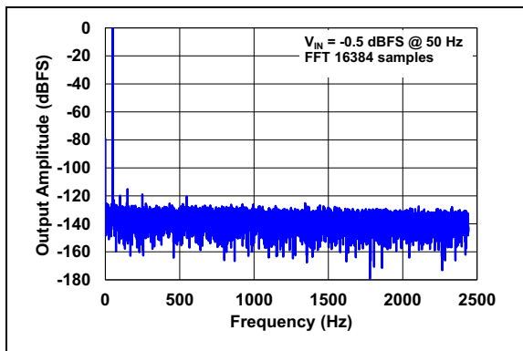
FIGURE 2-3: FFT Output Spectrum, f_{in} = 50\text{ Hz (Internal }V_{REF}\text{)} .
