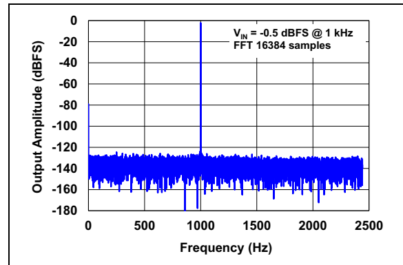
FIGURE 2-4: FFT Output Spectrum, f_{in} = 1\text{ kHz (Internal }V_{REF}\text{)} .
