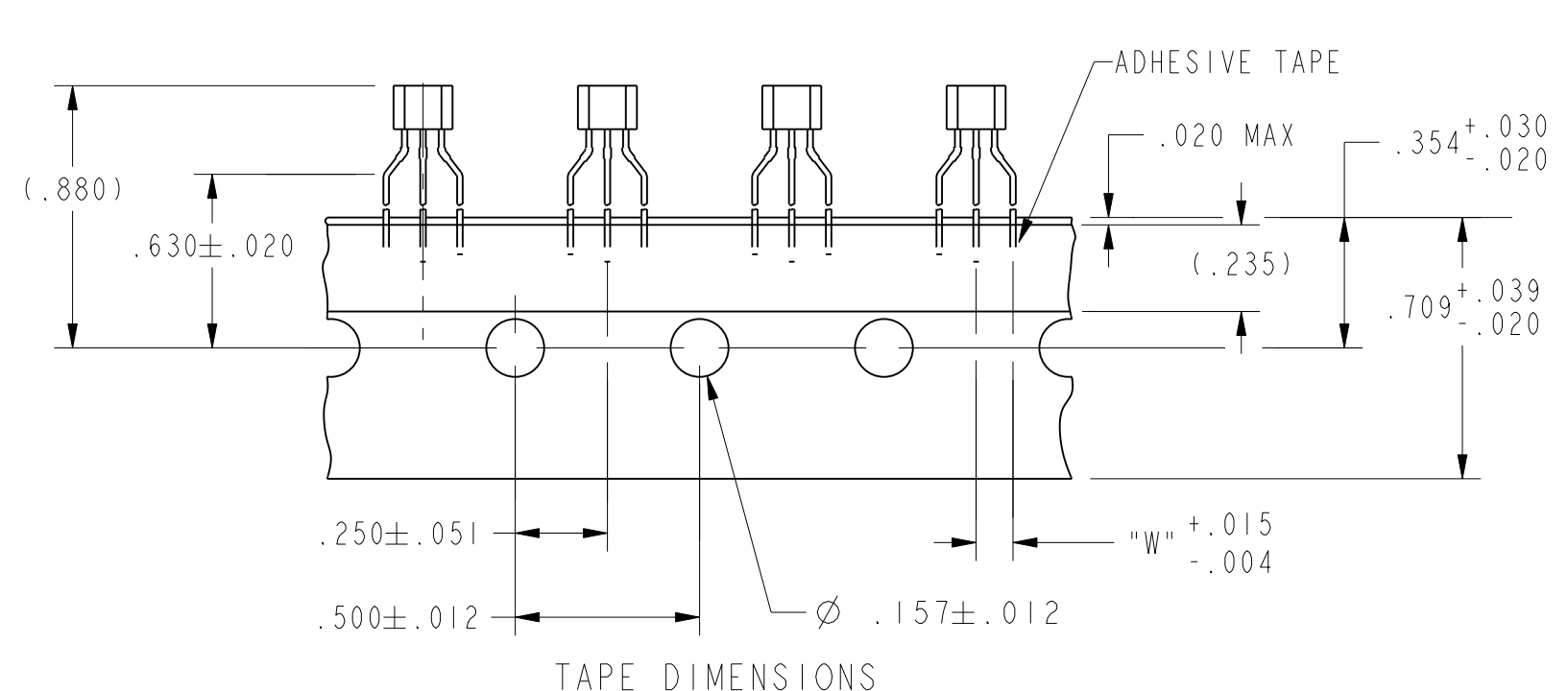
TAPE PACKING OPTIONS
