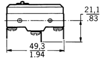
D6 .250" (6.35 mm) wide x .032" (0.81 mm) thick quick-connect
