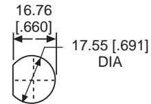
RECOMMENDED PANEL CUTOUT
