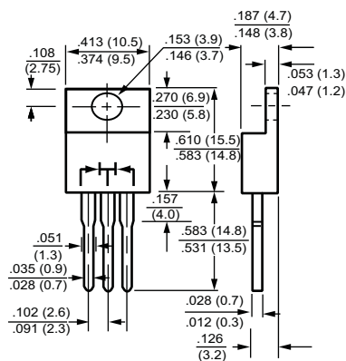
TO-220
