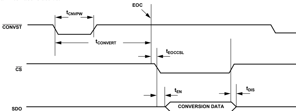
Figure 54. Serial Interface Read Timing in Normal Mode
