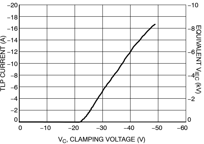
Figure 10. Typical Negative TLP IV Curve
