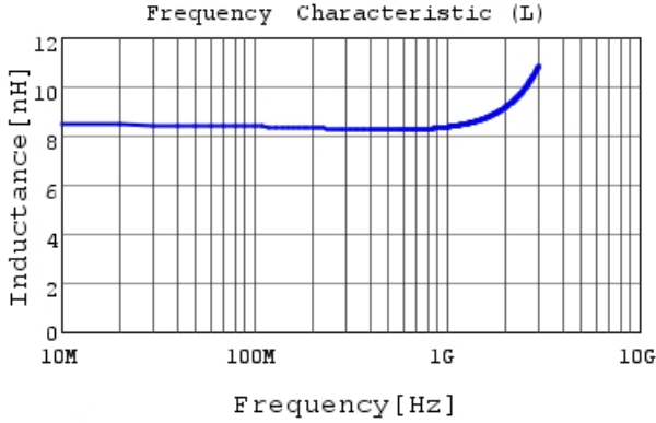
LQP15MN8N2B02 L
