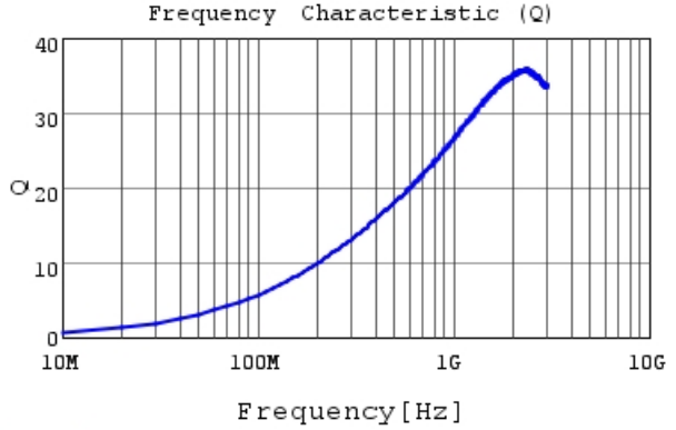
LQP15MN8N2B02 Q
