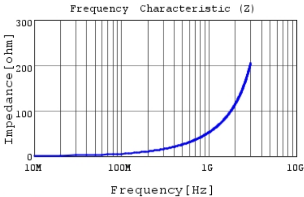
LQP15MN8N2B02 |Z|
