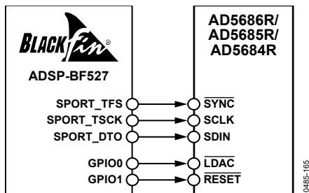
Figure 60. SPORT Interface
