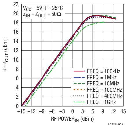
RF Power Out vs RF Power In Over Frequency
