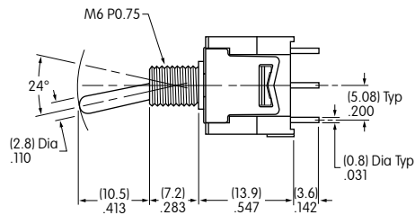
Actuator in Down Position
