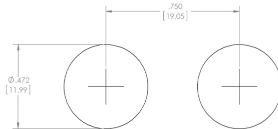
RECOMMENDED MOUNTING HOLE PATTERN
