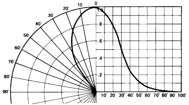
Figure 8: Relative Luminous Intensity vs. Angular Displacement, HLMP-K101
