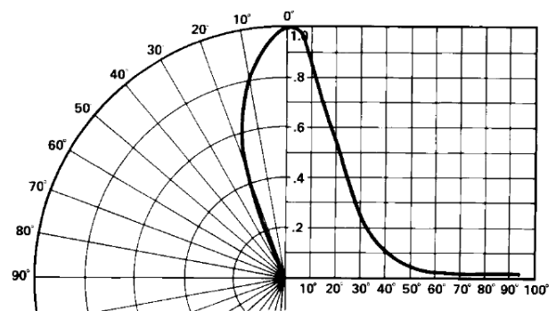
Figure 10: Relative Luminous Intensity vs. Angular Displacement, HLMP-K105
