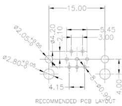
8 Contact PCB Layout
