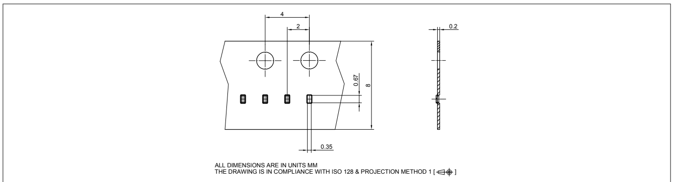
Figure 13 WLL-2-3 packing
