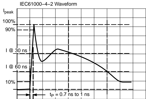
Figure 9. IEC61000–4–2 Spec
